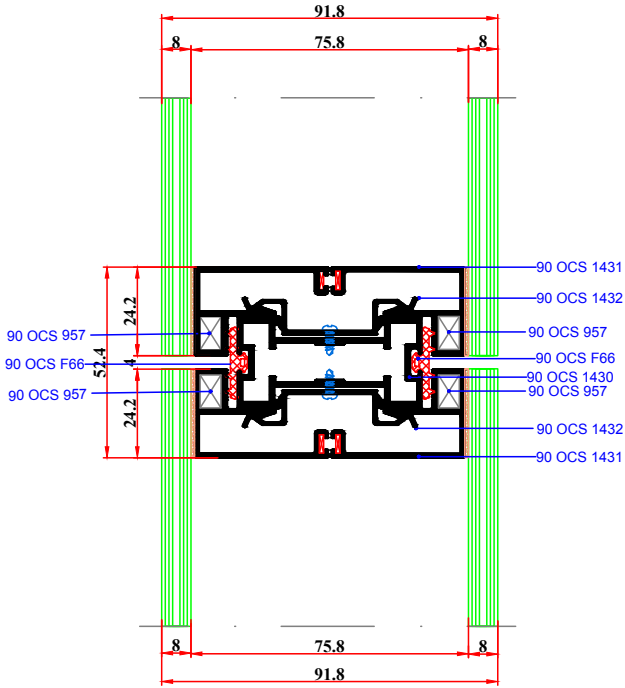
1 NOLU DETAY
