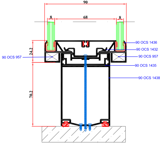
1 NOLU DETAY
