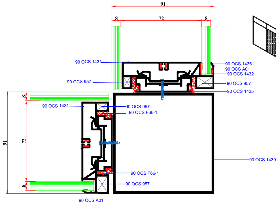
1 NOLU DETAY
